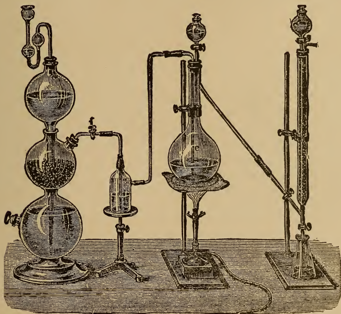
Fig. 107. APPARATUS FOR FINDING AND MEASURING SULPHUR.
